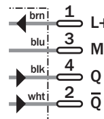
M8, 4-pin
