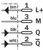
M12, 4-pin
