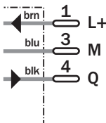
M8, 3-pin
