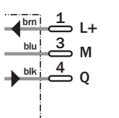
M8, 3-pin
